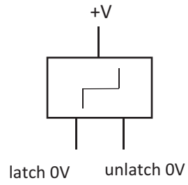
Latching relay coil
